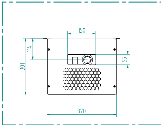
Cooling unit 1:10
